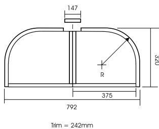
Type D - 790mm Wide (147 x 715mm Flat Door, code 17)
