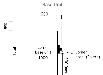
1000mm Conventional Corner Base Unit
