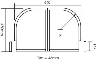
Type F - 640mm Wide x 470mm (147 x 715mm Door x 2, code 17)
