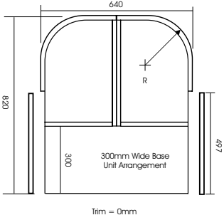
Type E - 640mm Wide x 820mm (497 x 715mm Door x 2, code 57)
