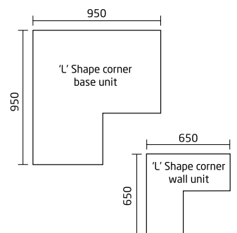
'L' Shape Corner Units Note:- Walls must be square to accommodate L shaped units.
