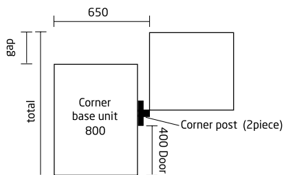
800mm Conventional Corner Base Unit
